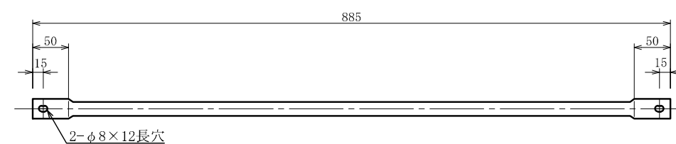
F-885 \phi 19 \times 885\ell
